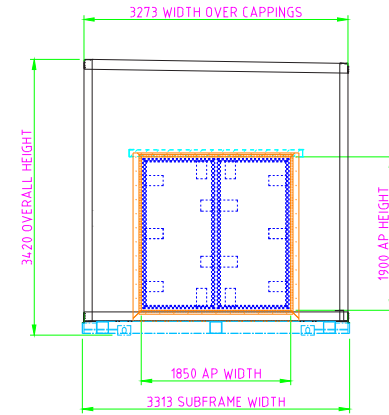
REAR VIEW OF ASSEMBLED BOX
