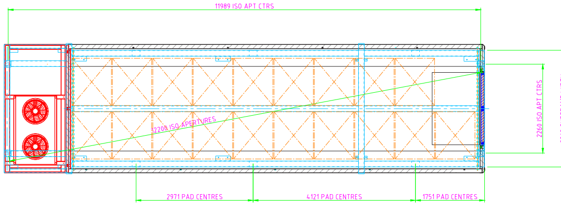
PLAN VIEW OF ASSEMBLED BOX
