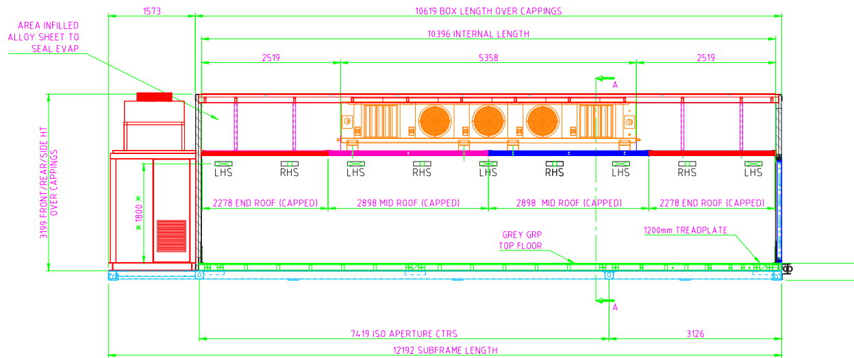
SIDE VIEW OF ASSEMBLED BOX
