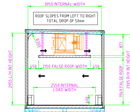
VIEW ON ARROWS A - A
