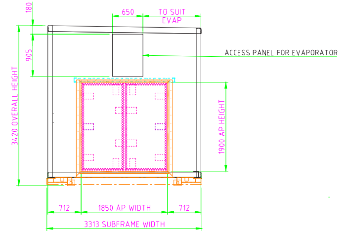
REAR VIEW OF ASSEMBLED BOX
