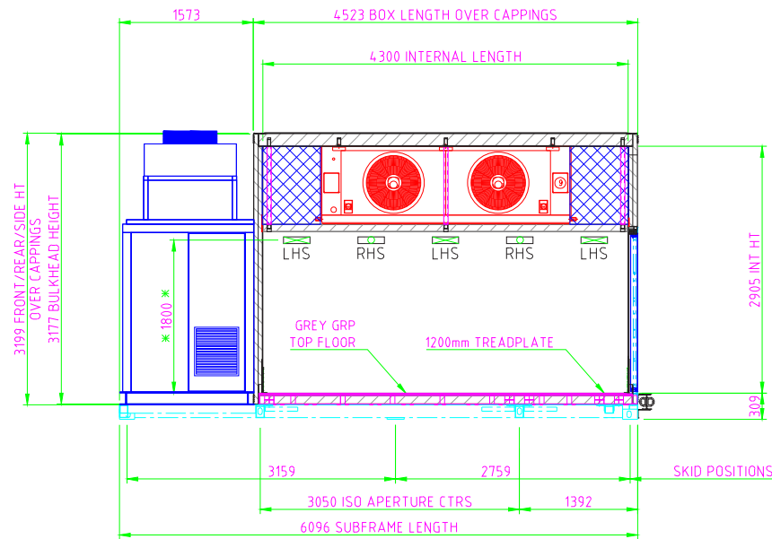
SIDE VIEW OF ASSEMBLED BOX
