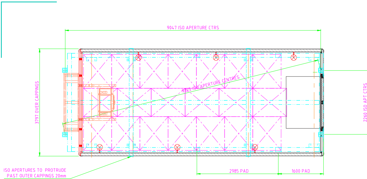
PLAN VIEW OF ASSEMBLED BOX
