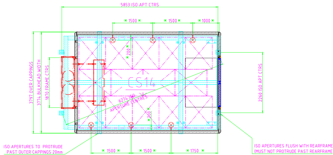
PLAN VIEW OF ASSEMBLED BOX
