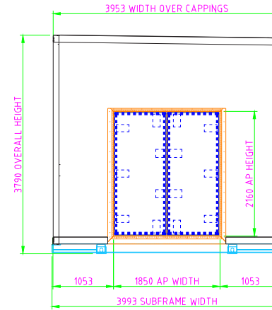
REAR VIEW OF ASSEMBLED BOX
